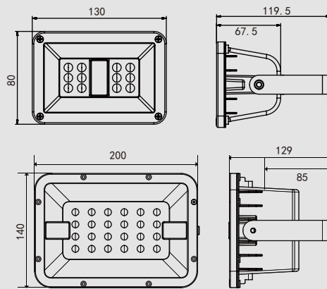
External Lamp (Flood Light)
